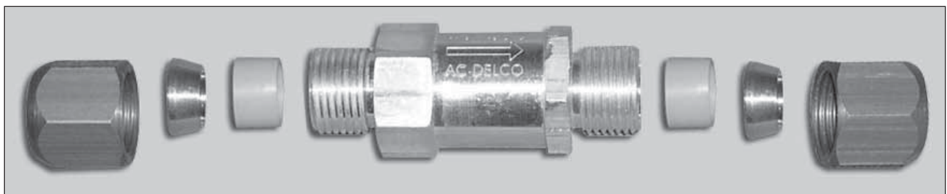
In-liquid-line filters can be installed to trap debris that may be in an A/C system after it has suffered a catastrophic compressor failure. Filters of this type are available from a number of different A/C parts suppliers.
