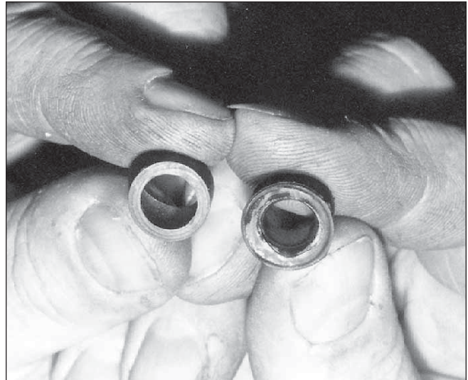
The seals on service equipment hoses must be frequently inspected for damage and replaced when necessary. This shows a comparison between a new seal (left) and a used one that is swollen and distorted (right).
