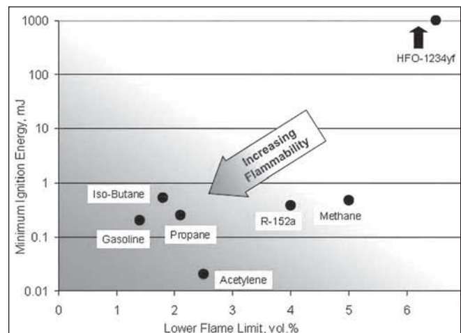
Comparison of energy required to ignite various chemical mixtures. (W Hill & SAE Int'l)
