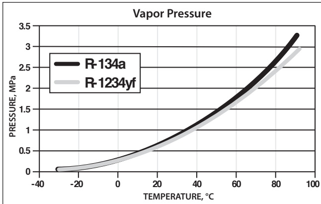
Vapor pressures for the two refrigerants are very similar except at extreme pressures.
