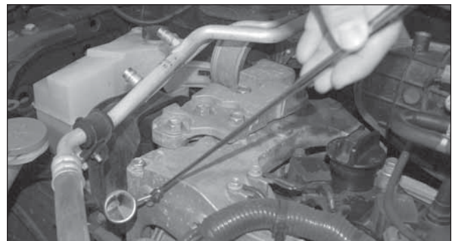
You can use a mirror to reflect the UV light underneath components in hard to see locations. If dye is present at a leak site, you should see it glowing.
