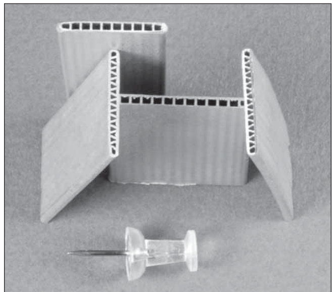
Today's condensers have very tiny refrigerant multi-flow passages. Not only can't you even fully insert a toothpick into some of them, others are so small, a push pin will barely go in. This is why attempts to flush debris-dogged condensers are often not successful.
