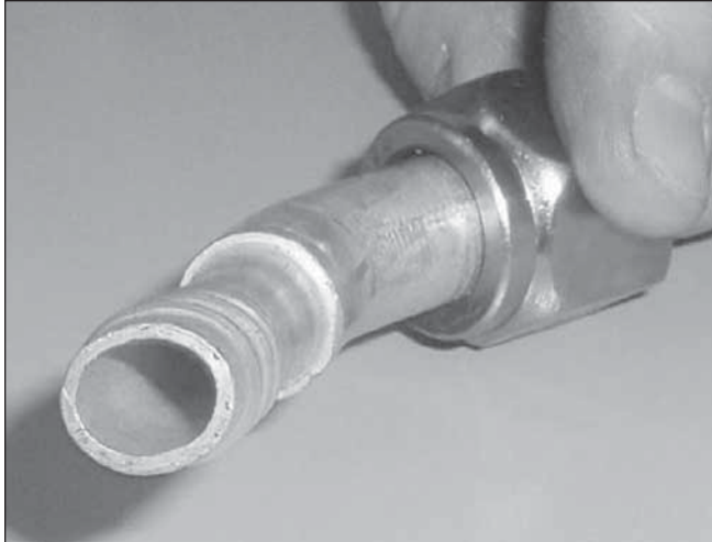
Incorrect tube and hose combination causing tube to seriously deform.
