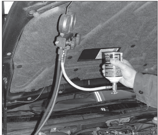
Some technicians still attempt to use small cans and pressure gauge readings to charge systems, but accurate charging is not possible with this method.
