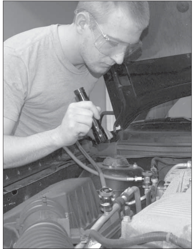
Like this technician, always be sure to wear the special goggles that came with your UV dye leak detection kit. Not only do they protect your eyes from the UV light, they also make dye traces at leak sites stand out better.
